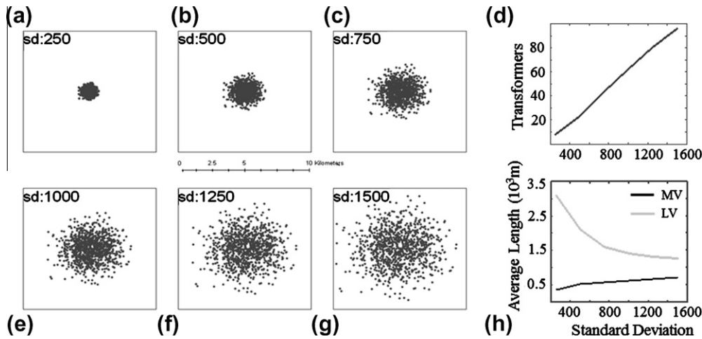
Fig. 12. Multivariate normally distributed random data and results: a–c and e–g, multivariate normally distributed 10 \times 10 \text{ km}^2 sites with 1000 demand points. (d) The behavior of algorithm as the standard deviation increases. (h) Average LV line per transformer declines as the average MV line and the number of transformer increases.
