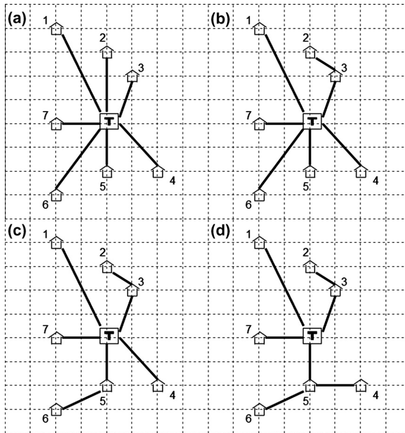
Fig. 6. A seven-point example of Essau-William's CMST algorithm: (a) Initial star configuration. (b) Maximum trade-off value is for Point 1 (2.23) however it violates L_{\max} . Point with the next best trade-off value (Point 2) is selected. (c) Next best trade-off value is for Point 6. (d) Final configuration is reached after Point 4 is connected.
