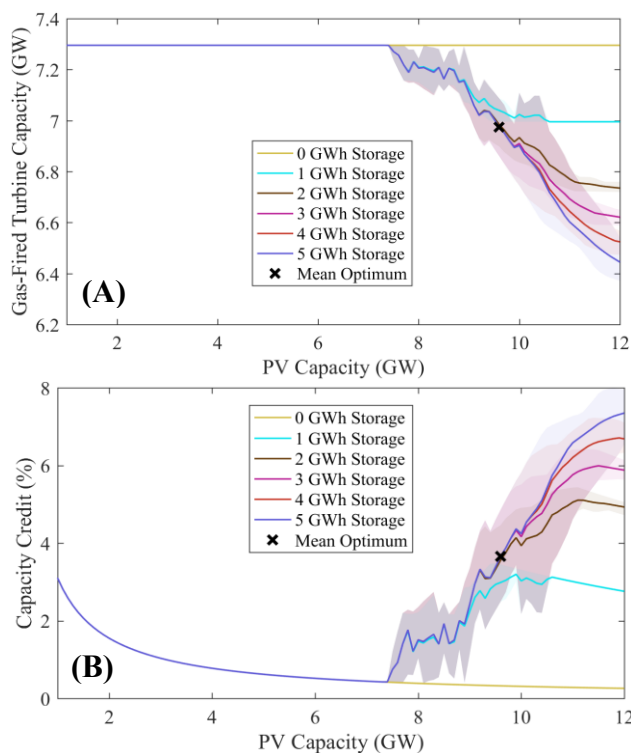
Fig. 7. Effects on gas-fired turbine capacity A) peak demand; B) Capacity credit
