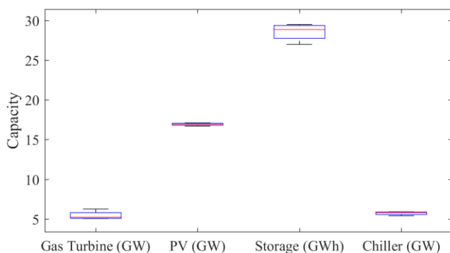
Fig. 11. Scenario 2 optimum range of gas turbine, PV, storage and chiller capacities using 4 years of solar data
