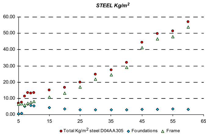
Fig. 7. Quantity of steel in the foundations and frame (kg/m 2 ).
