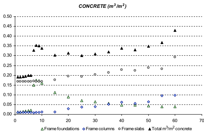
Fig. 8. Quantity of concrete in the foundation, frame and total (m 3 /m 2 ).
