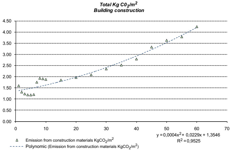
Fig. 9. Emissions due to construction materials (kg CO 2 /m 2 ).
