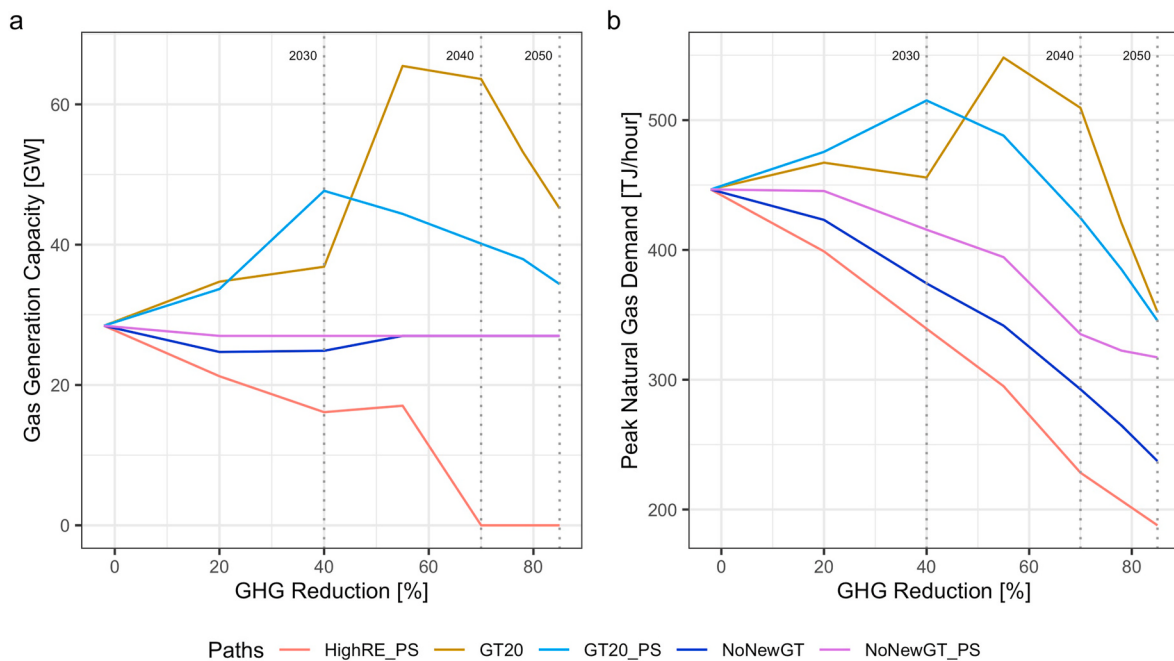
Fig. 4. | NYS decarbonization pathways showing (a) gas generation capacity, (b) maximum statewide natural gas demand. “GT20” indicates 20-year GT capital cost annualization; “PS” indicates scenarios with peak shaving.
