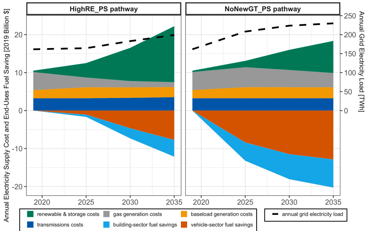
Fig. 6. | Annual electricity supply cost and end-uses fuel cost saving (area chart, left y-axis. Supply cost as positive and savings as negative) and annual grid electricity load (dashed line, right y-axis) from 2019 to 2035 of New York State HighRE_PS and NoNewGT_PS pathways. End-Uses electrification increases electricity load as well as decreases directly fossil fuel consumption. In the cost categories, “renewable & storage” represents all costs related to onshore and offshore wind, utility-scale solar, utility-scale battery; “gas generation” represents all costs related to fossil fuel generation; “baseload generation” represents all costs related to nuclear, hydropower, imported hydropower, and biofuel generation; “building-sector fuel” represents propane, fuel oil, and natural gas in building sector; “vehicle-sector fuel” represents diesel and gasoline in vehicle sector.
