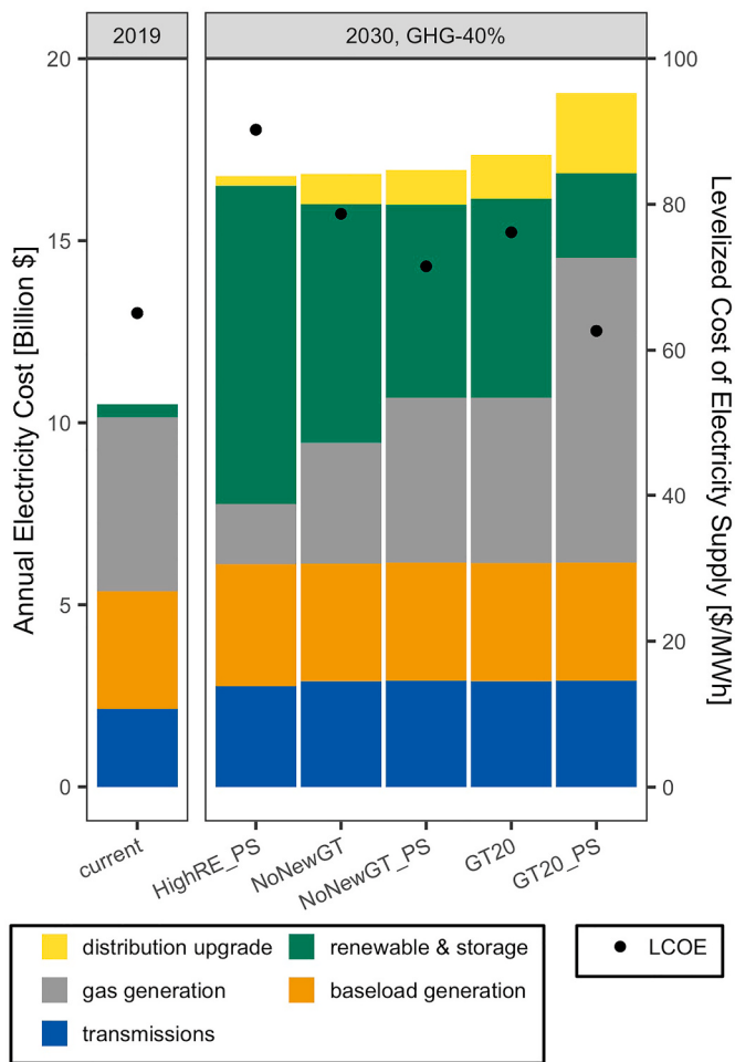
Fig. 5. | Sectoral annualized cost of electricity supply (bars, left y-axis) and levelized cost of electricity (LCOE) supply (points, right y-axis) of different New York State decarbonization pathways. “GT20” indicates 20-year GT capital cost annualization; “PS” indicates scenarios with peak shaving. Results are shown for the current grid system and pathway results corresponding to 2030. In the cost categories, “distribution upgrade” represents the demand-side distribution expansion costs due to electrification; “renewable & storage” represents all costs related to onshore and offshore wind, utility-scale solar, utility-scale battery; “gas generation” represents all costs related to fossil fuel generation; “baseload generation” represents all costs related to nuclear, hydropower, imported hydropower, and biofuel generation.
