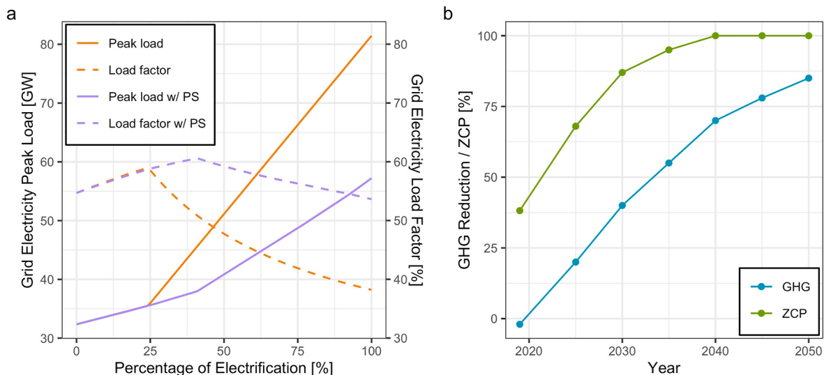
Fig. 1. | (a) Statewide electricity load peak (left y-axis) and load factor (right y-axis) with and without peak shaving (PS); (b) GHG emissions reductions and zero-carbon electricity percentage (ZCP) for the simulated decarbonization pathways.
