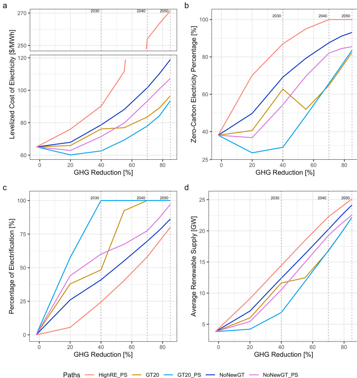
Fig. 3. | NYS decarbonization pathways showing (a) levelized cost of electricity, (b) zero-carbon electricity percentage, (c) building and vehicle electrification rate, and (d) total average renewable electricity supply (including behind-the-meter solar photovoltaic projected in the model). “GT20” indicates 20-year GT capital cost annualization; “PS” indicates scenarios with peak shaving.
