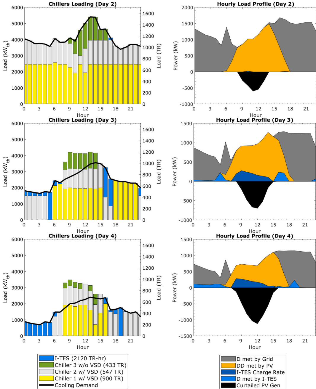
Fig. 13. Cost-optimal system with (a) chillers loading and (b) hourly load profile without carbon pricing.
