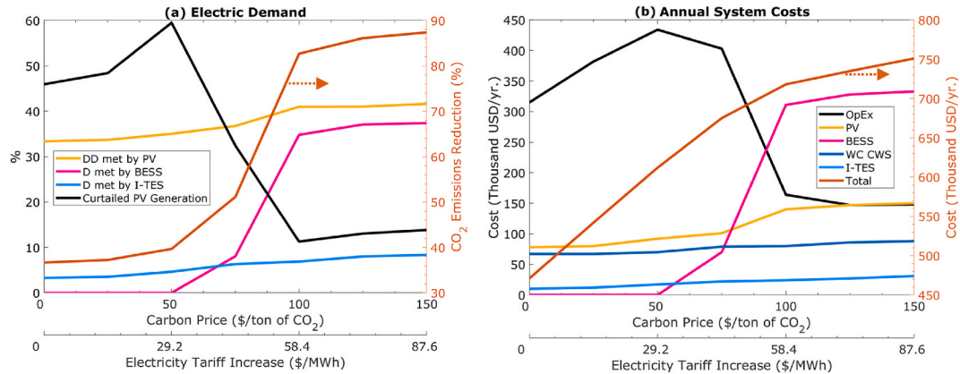
Fig. 11. Effect of the carbon price increases on (a) contribution to meeting the electric demand and (b) breakdown of annual system cost.
