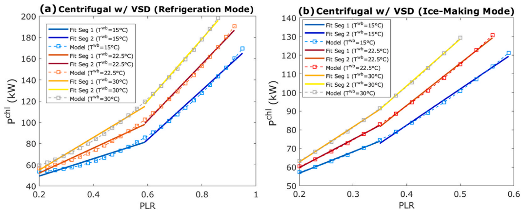
Fig. 4. Illustration of piecewise linearized chiller performance curve for 383-ton Carrier 19XR chiller with VSD centrifugal compressor under three ambient wet-bulb temperatures in (a) refrigeration mode with a setpoint temperature of 7^\circ\text{C} , and (b) ice-making mode with a setpoint temperature of -6^\circ\text{C} .
