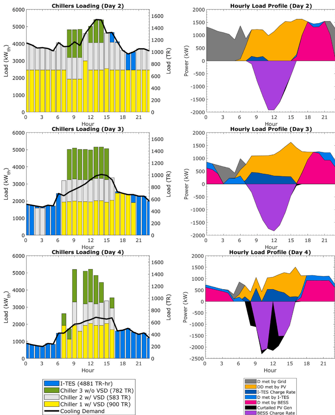
Fig. 14. Cost-optimal system with (a) chillers loading and (b) hourly load profile with carbon pricing at $100/ton of CO 2 .
