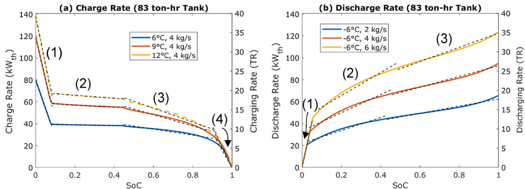
Fig. 6. Piecewise linearized (a) charge and (b) discharge rates for a generic CALMAC 83-ton-hr I-TES.
