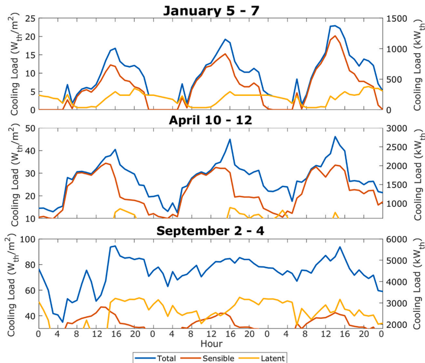
Fig. 8. Simulated residential building cooling load for three days in winter, spring, and summer. Electric and thermal loads are correlated with higher building occupancy in the evening.
