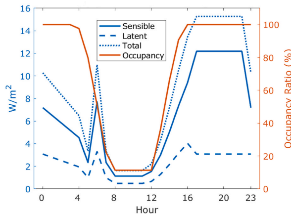
Fig. 7. Estimated residential building non-cooling electric load.
