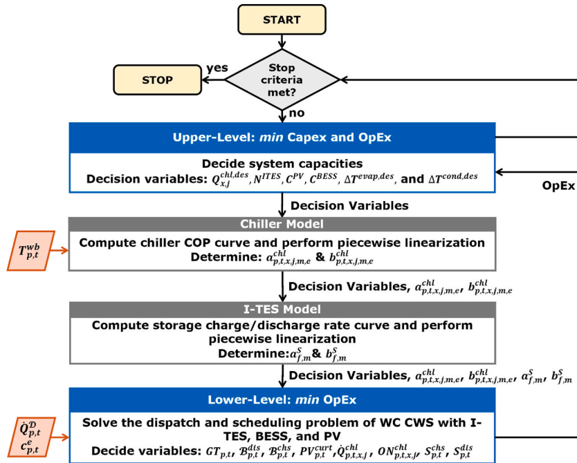
Fig. 2. Bi-level optimization formulation. The upper level minimizes annual system costs and decides the installed capacities and the lower level solves the equipment scheduling and dispatch problem in a mixed-integer linear programming formulation and returns system electricity use.
