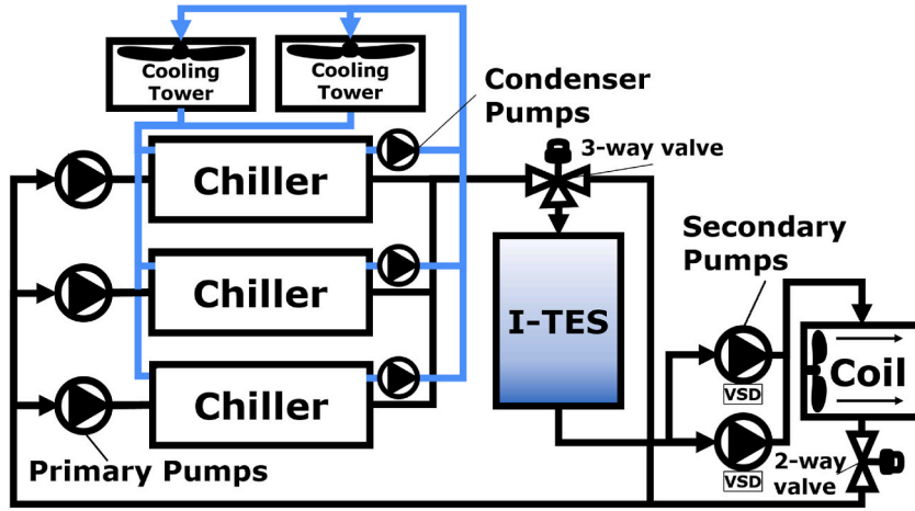
Fig. 3. Chilled water system in a primary-secondary flow configuration.
