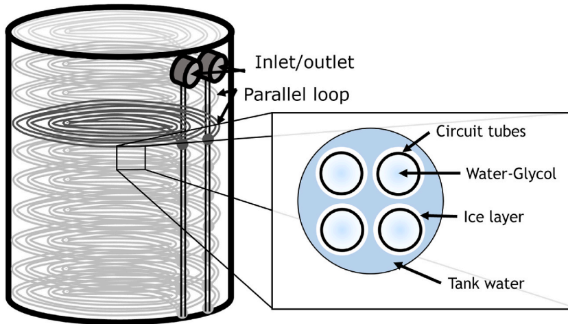
Fig. 5. An illustration of a modular internal melt I-TES. Multiple parallel circuits are submerged in water inside the tank, and a water-glycol mixture is circulated through the circuits to build and melt the ice around the tubes.
