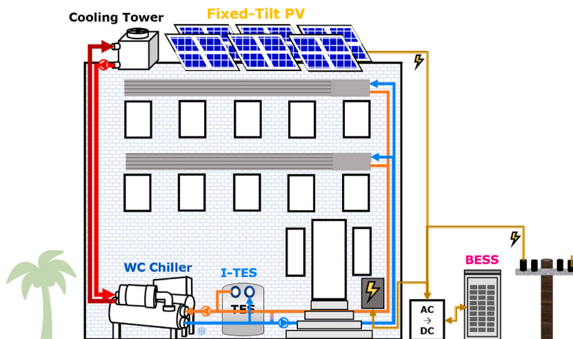
Fig. 1. A schematic of an integrated WC CWS with I-TES, BESS, and on-site PV generation.
