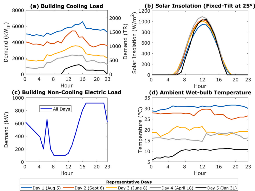
Fig. 9. Selected five scenarios with (a) building thermal cooling demand, (b) solar insolation, (c) non-cooling electric load, and (d) ambient wet-bulb temperature.
